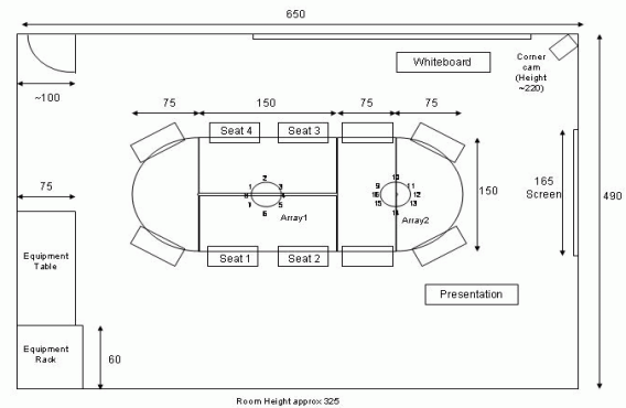
Fig. 1. The layout of the UEDIN Instrumented Meeting Room (measurements in cm). Array microphones are numbered 1-16. Cameras are mounted under Array 1 to give closeup views of participants in the seated locations. The six reading locations are indicated as Seat 1-4, Presentation and Whiteboard.
